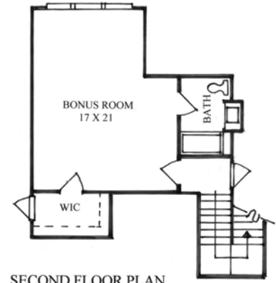
SECOND FLOOR PLAN HEATED SQ. FT. 498
